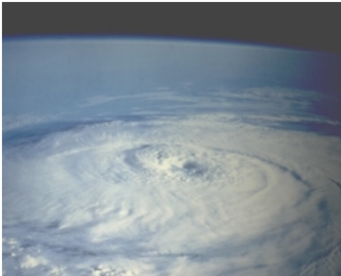
Light from the sun provides heat that drives atmospheric winds and ocean currents on Earth's surface.
